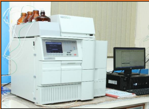
High Performance Liquid Chromatography- Photo Diode Array
